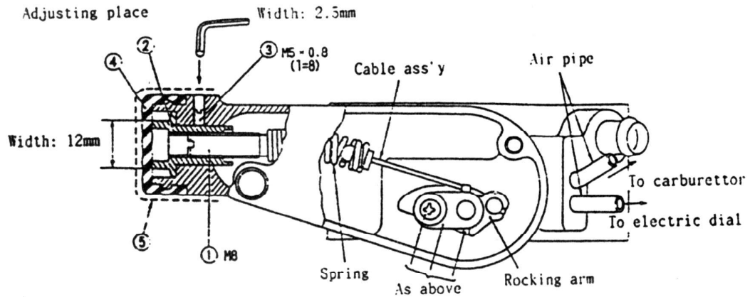
Fig.1-2 Regulator
